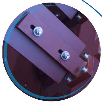
MIXING BLADES IN HARDOX 500 HB 20 MM (0.8 INCH) THICKNESS, HIGHLY CRASH-PROOF. MIXING BEAMS IN SPHEROIDICAL IRON BOLTED TO THE SHAFTS
