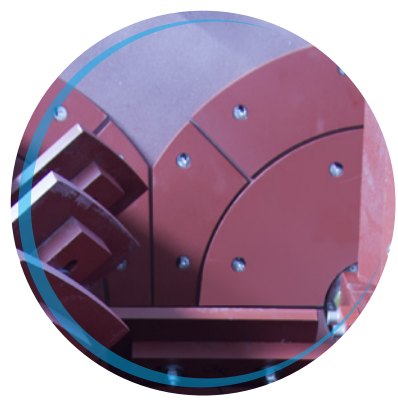
BIN COAT HARDOX 500 HB 12 MM (0.5 INCH) THICKNESS. OFFSET RECTANGULAR PLATES. AS OPTION, THE COATING CAN BE SUPPLIED IN HARDOX 500 HB 15 MM (0.6 INCH)
