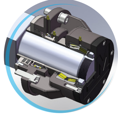
HARDENED COLLETS TO PROTECT THE MIXING SHAFT. SEALING SYSTEM COMBINED WITH POLYURETHANE COLLARS AND MECHANICAL SEALS GROUND STEEL
